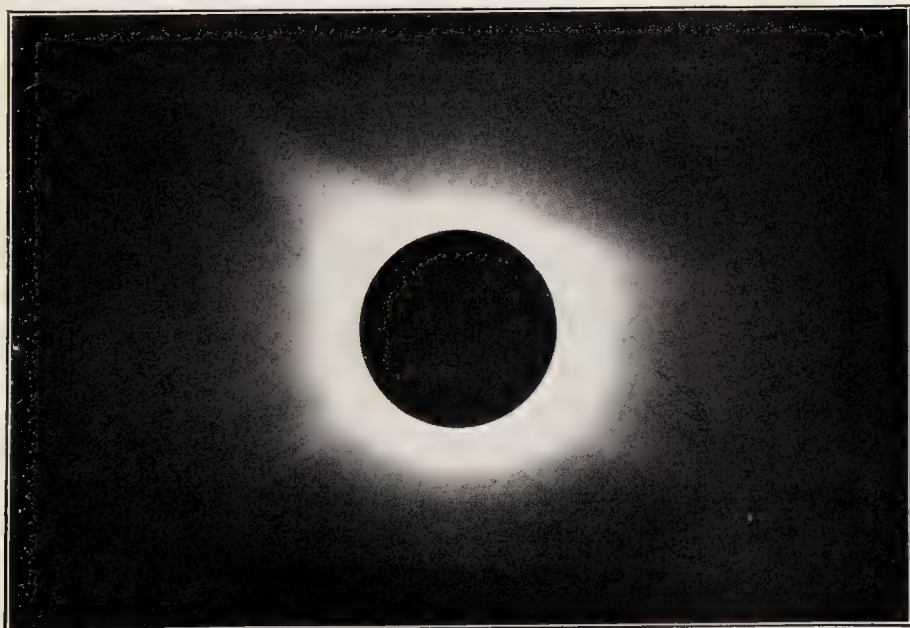
SOLAR CORONA OF 1922
